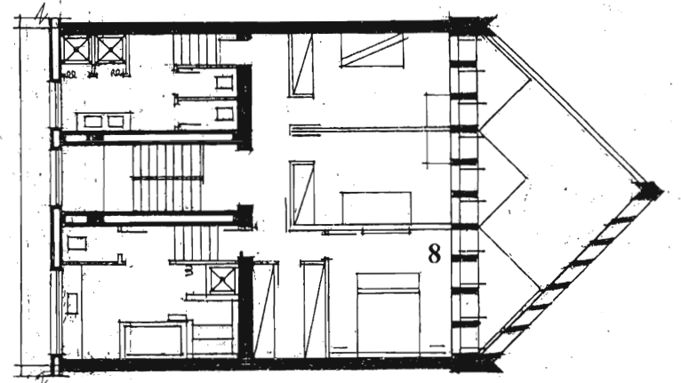
Plan of 3 rd and 3 1/2 levels
