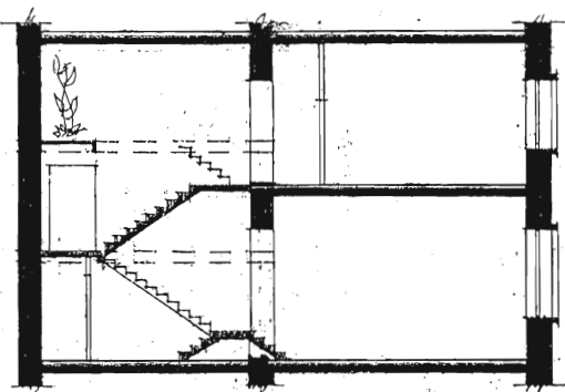
SECTION 1 - 1
