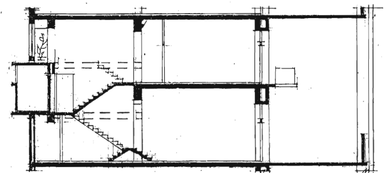
SECTION 1 - 1
